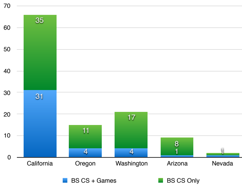
Degree Distribution
